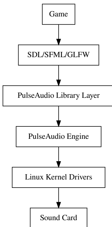
Figure 131: How many abstraction layers are used just for a game to be able to play sounds
